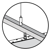
Aluminum Channel with Adjustable Cable Gripper • Clear anodized finish (matte black available) • Suspension point pre-mounted but can be repositioned on site
