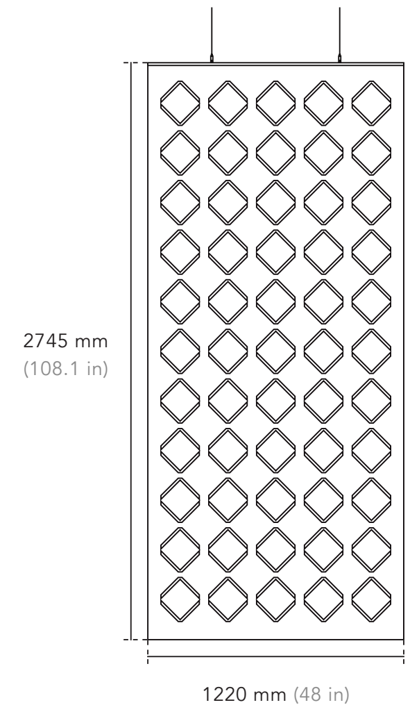
DMD-SC-122-274 (11% of panel cut out)
