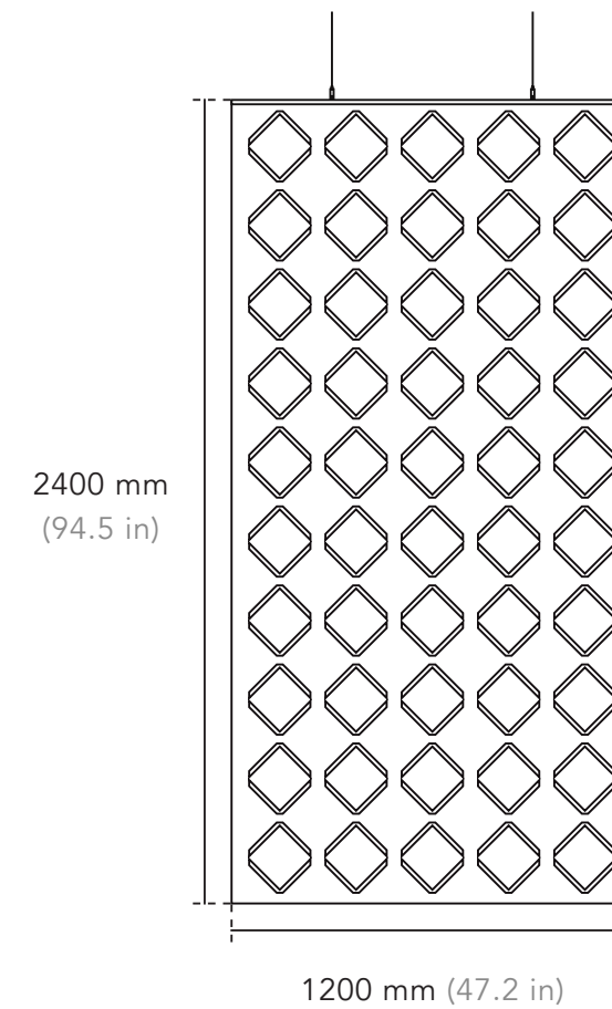
DMD-SC-120-240 (12% of panel cut out)
