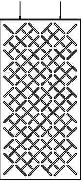
LTC-SC-120-240 (18% of panel cut out)
