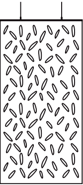
SED-SC-120-240 (18% of panel cut out)
