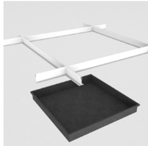
Box ceiling tile with extended edge
