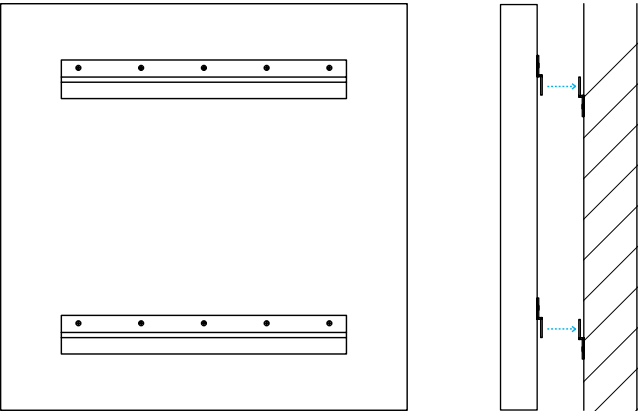
Z-CLIPS
